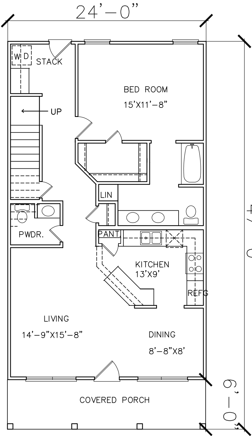
LOWER LEVEL FLOOR PLAN
