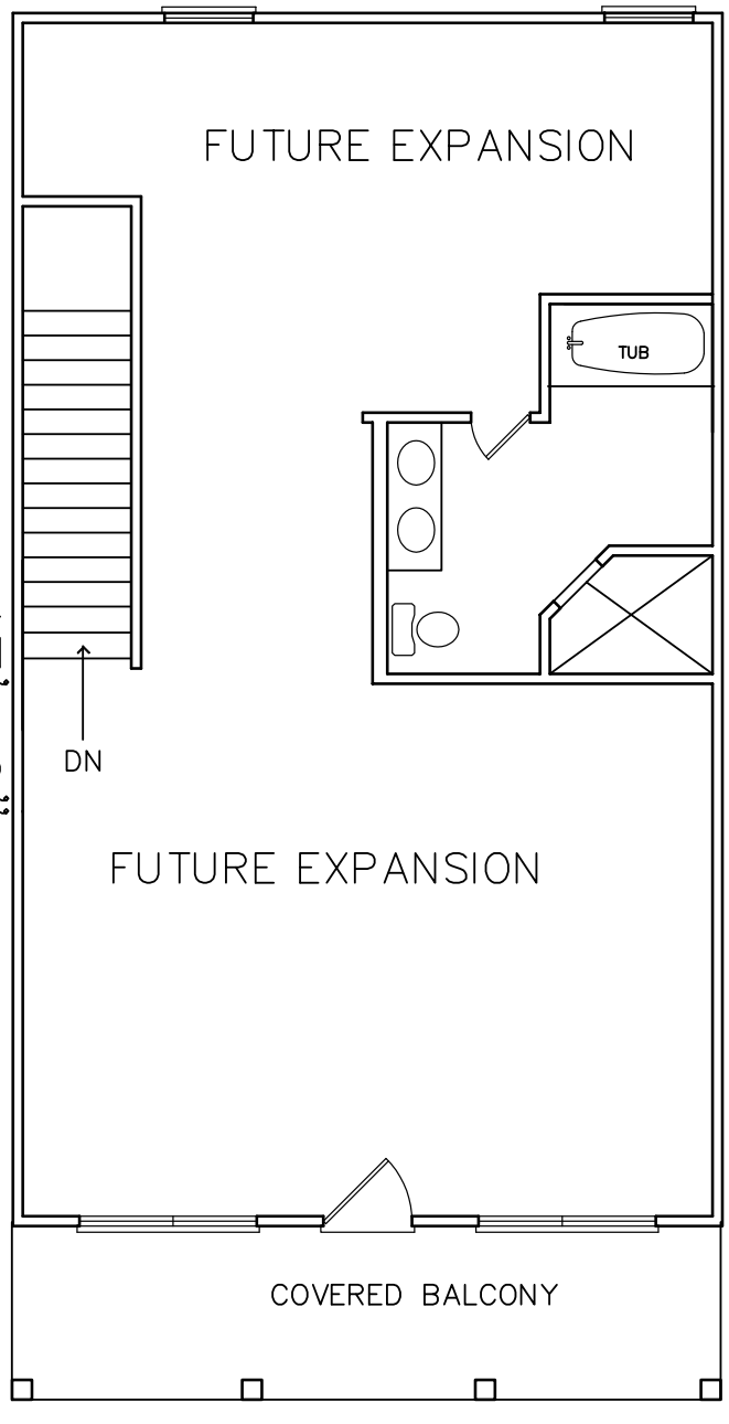
UPPER LEVEL FLOOR PLAN
